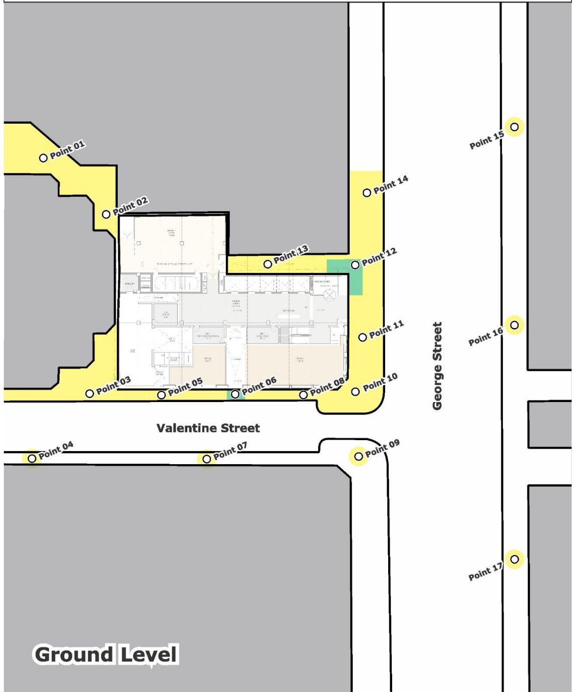
Figure 5: Study Point Locations and Target Wind Speed Criteria - Ground Level
